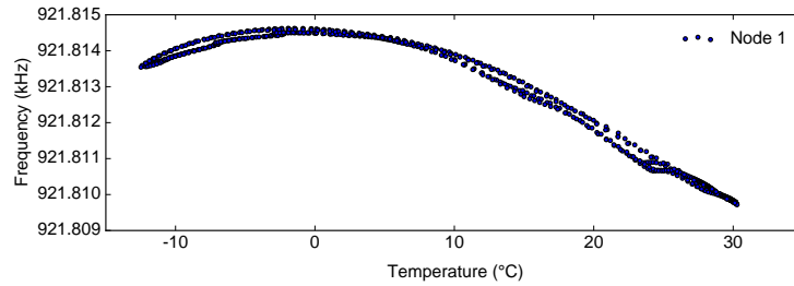
Fig. 3. Hardware clock frequency for a Mica2 node for different ambient temperatures [28].
