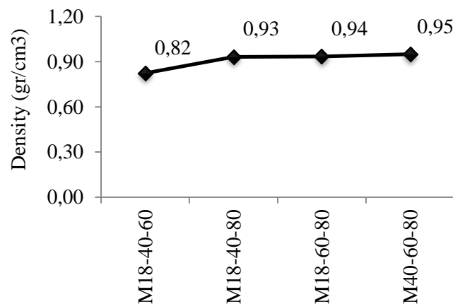
Figure 1. The effect of the filler meshes combination on particle board density
