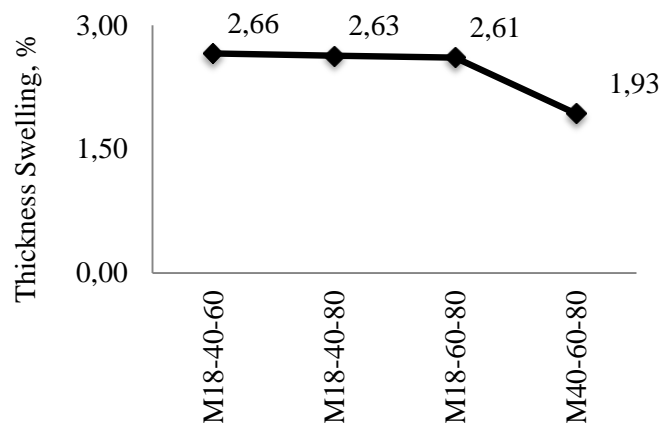
Figure 2. The effect of the filler mesh combination on the thickness swelling of the particle board
