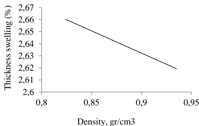
Figure 3. Correlation between density and thickness swelling of particle board
