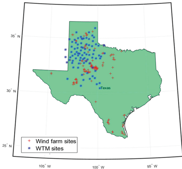
Fig. 2. West Texas Mesonet stations and ERCOT wind farms.
