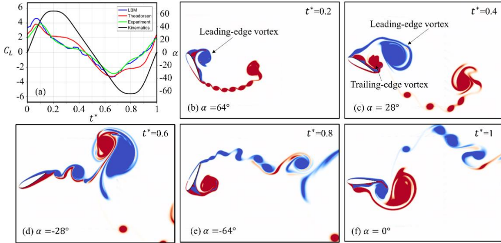
Figure 6. Comparison of the lift coefficient with experimental results and Theodorsen's theory (a); Time evolution of wake on the surface of the airfoil (b-f).
