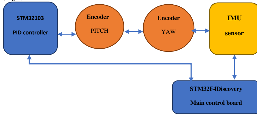
Fig.3. Automatic control system diagram
