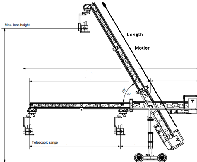
Fig.1. Crane structure and camera crane kinematics
