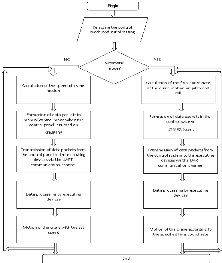
Fig.6. Compatibility and consistency manual and automatic control modes
