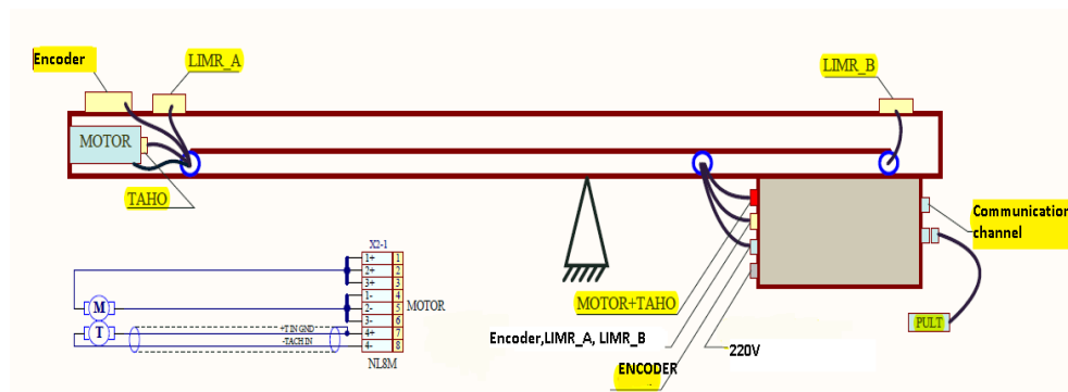
Fig.2. Control system with encoders
