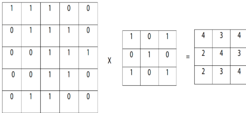
Figure 3.4: Convolutional Layer
