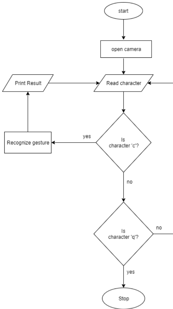
Figure 3.2: Flowchart of the recognition system
