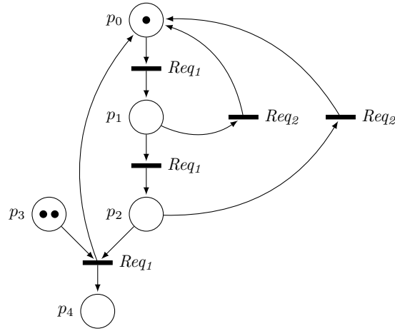
Figure 7: Pattern \Omega_3(3, 2) : two occurrences of three consecutive requests Req_1 : accepting marking M , M(p_4) = 2 .
