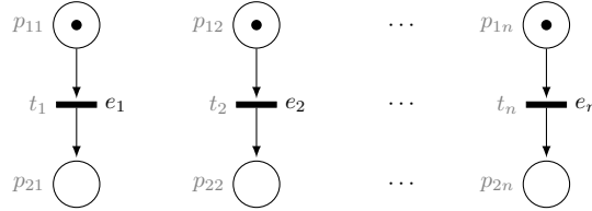
Figure 4: Pattern ( \Omega_2 ) about the occurrence of n events in no fixed order with the final markings Q_{\Omega_2} = \{p_{21}, p_{22}, \dots, p_{2n}\} .
